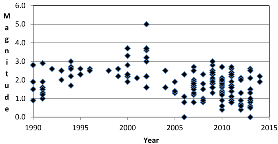
Figure 1. Plot of earthquakes and magnitude by year for occurrences within 100 miles of Sandgate, Vermont. Source: Northeast Earthquake Maps and Catalog 2015
